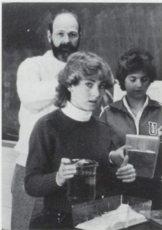
Above: Missy Boland doing an experiment on topographic contour lines.
